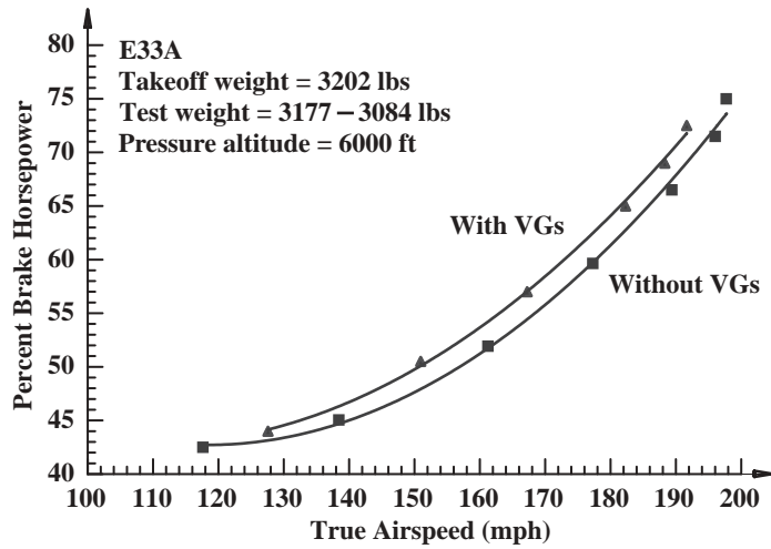
Figure 3. Percent brake horsepower versus true airspeed.
